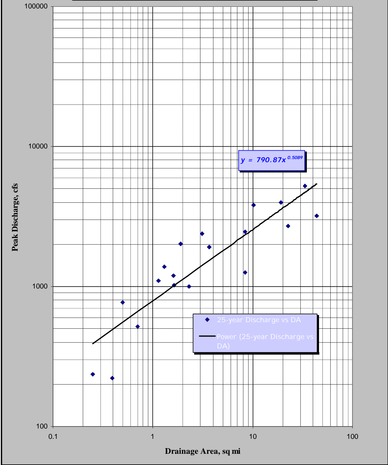
Figure 5. 25-yr Peak Discharge vs Drainage Area - Santa Cruz River Tributaries.
